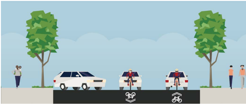
Figure 4: Minor Arterial Conceptual Cross Section 2
